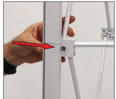
2. Lock the four center hubs
